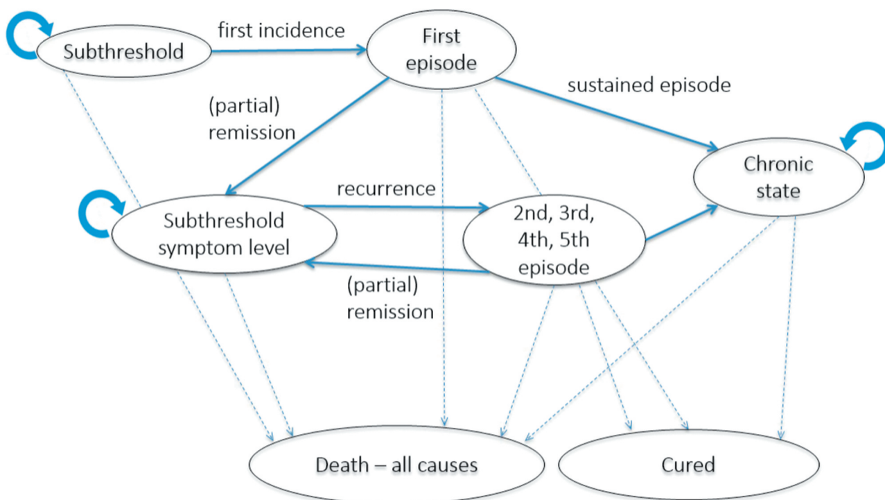
Figure 3. Markov-model.
